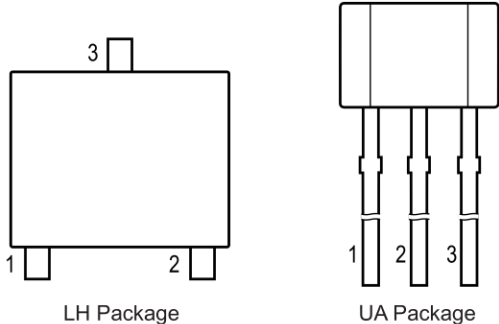
Pinout Diagrams
