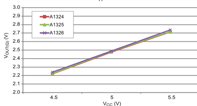
Quiescent Voltage Output versus Supply Voltage T_A = 25^\circ\text{C}
