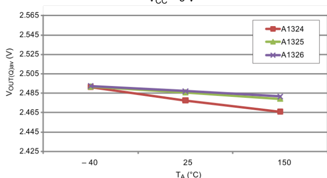
Average Absolute Quiescent Voltage Output versus Ambient Temperature V_{CC} = 5\text{ V}
