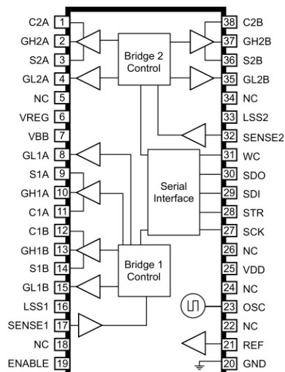
PINOUT DIAGRAM
