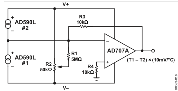
Figure 18. Differential Measurements
