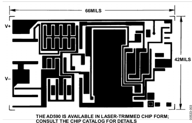
Figure 5. Metallization Diagram
