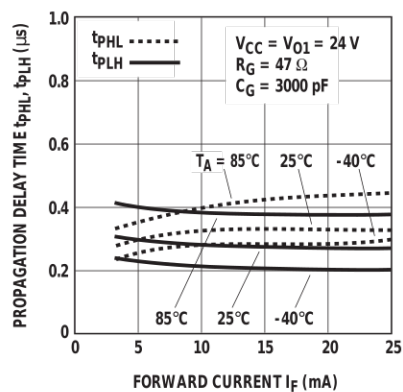
Figure 42. Typical propagation delay time vs. forward current, HCPL-3101.
