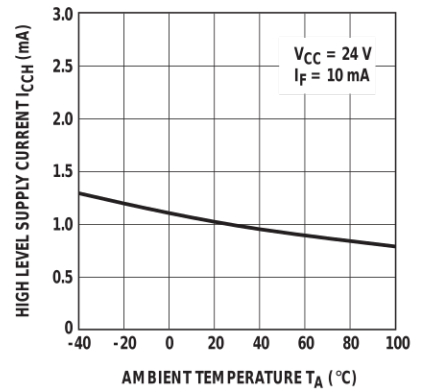
Figure 37. Typical high level supply current vs. ambient temperature, HCPL-3100.
