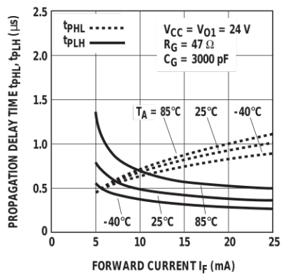
Figure 41. Typical propagation delay time vs. forward current, HCPL-3100.
