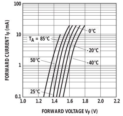
Figure 16. Typical forward current vs. forward voltage, HCPL-3101.
