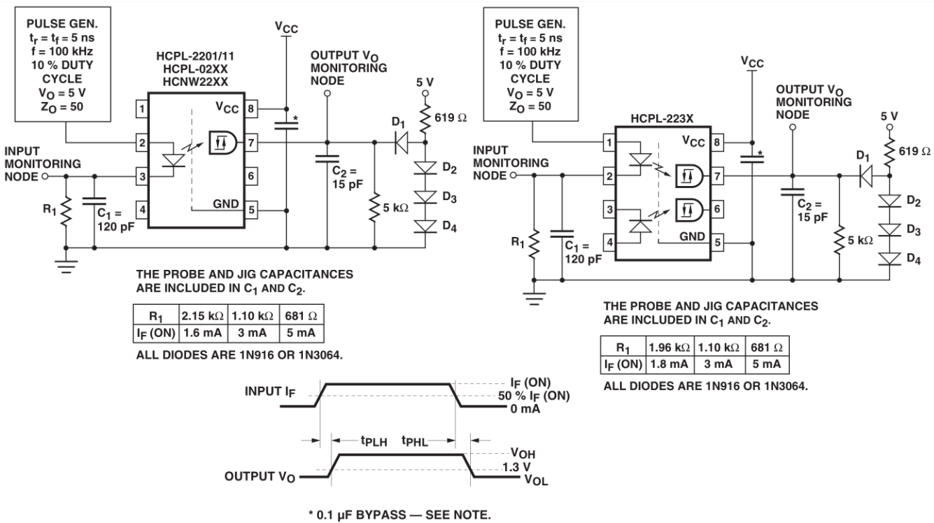
Figure 5: Circuit for t_{PLH} , t_{PHL} , t_r , t_f
