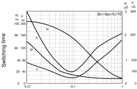
Switching Speeds
