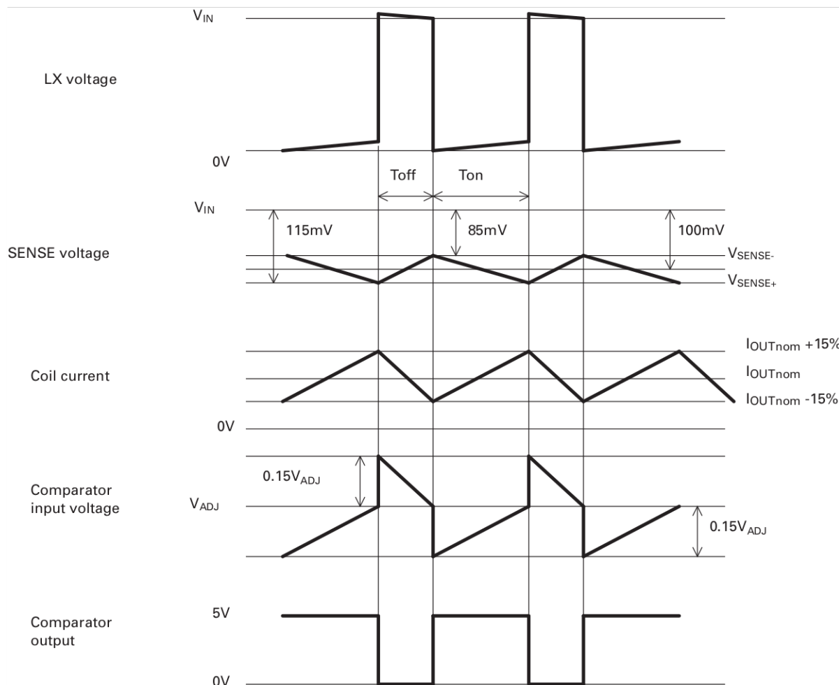
Figure 1 Operating waveforms
