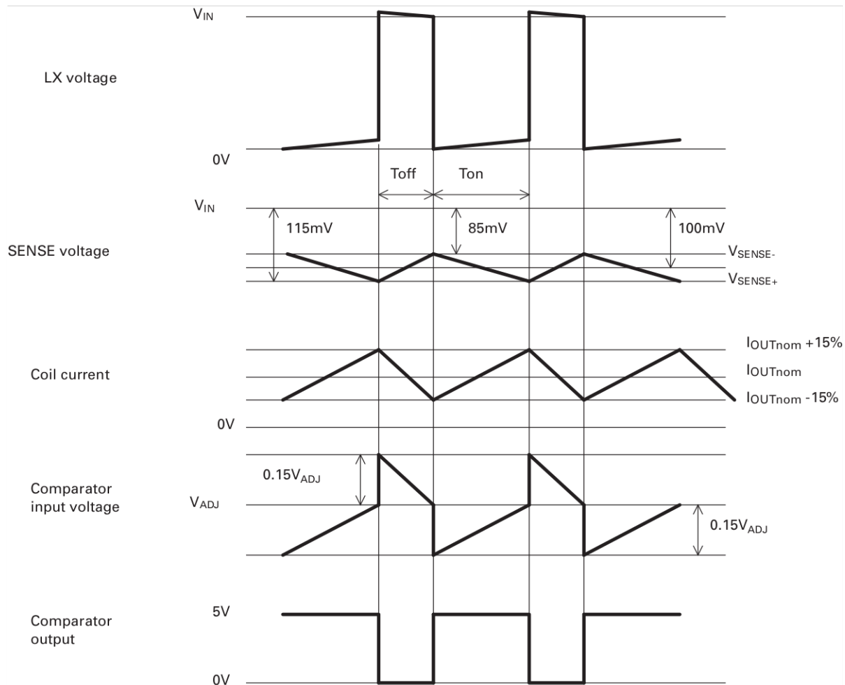
Figure 1 Operating waveforms
