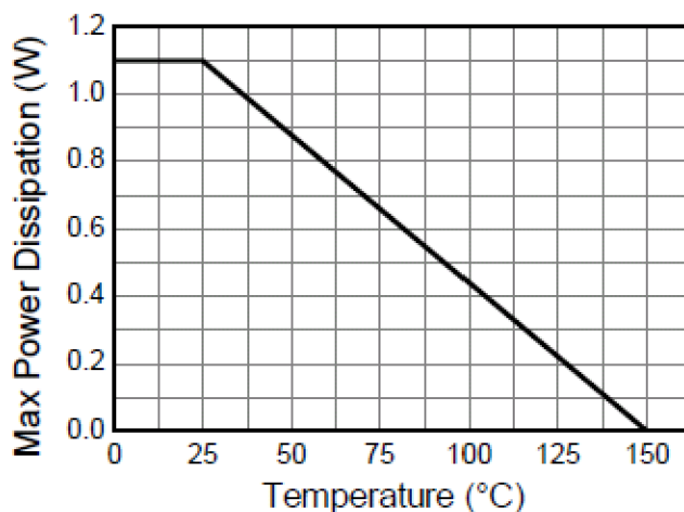
Derating Curve
