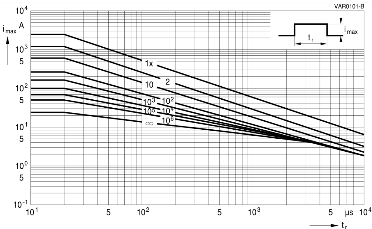
SIOV-S10K50 ... K320
