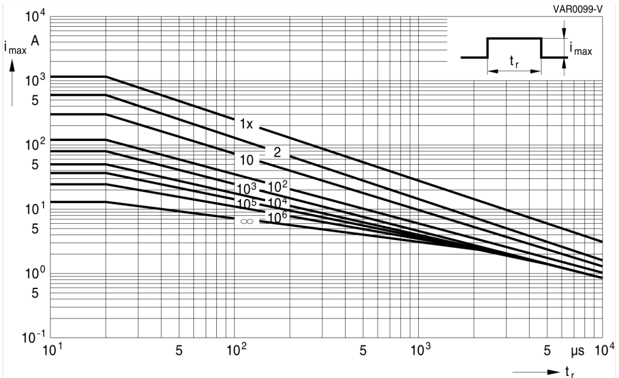
SIOV-S07K50 ... K460
