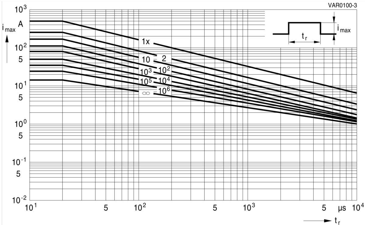
SIOV-S10K11 ... K40
