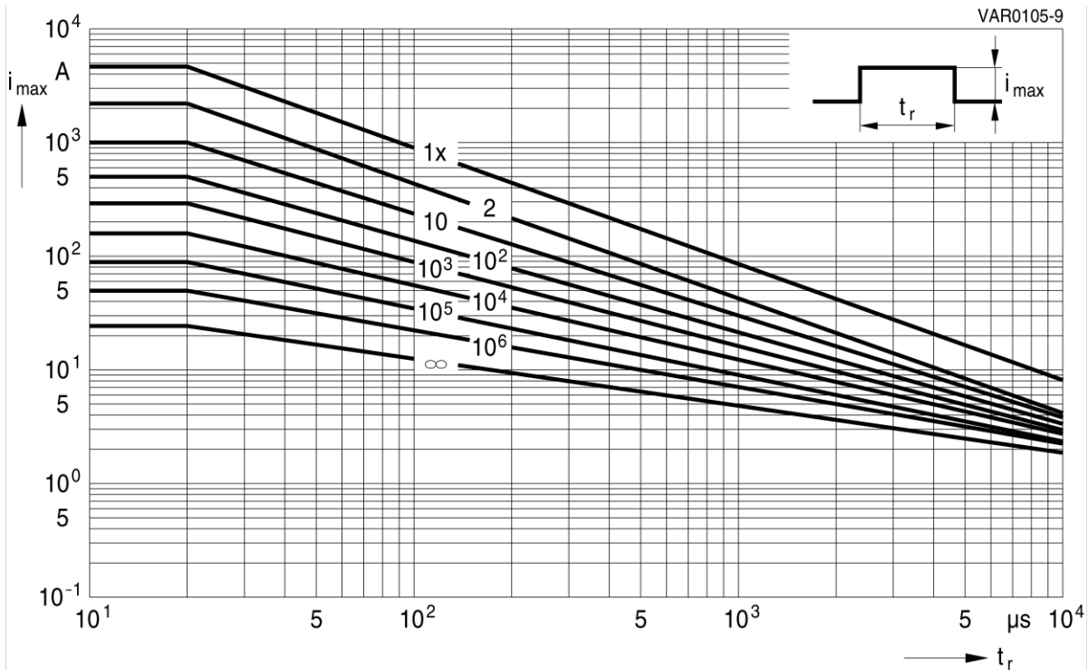
SIOV-S14K385 ... K1000
