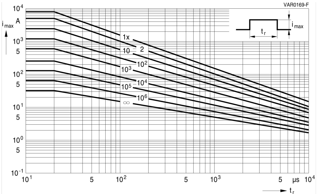
SIOV-S20K385 ... K460
