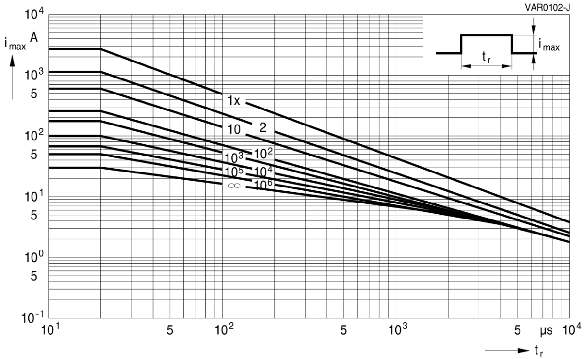
SIOV-S10K385 ... K680
