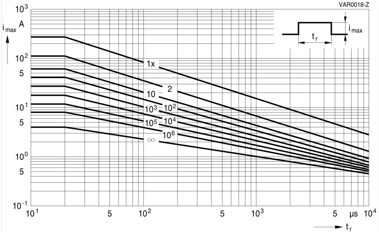
SIOV-S07K11 ... K40
