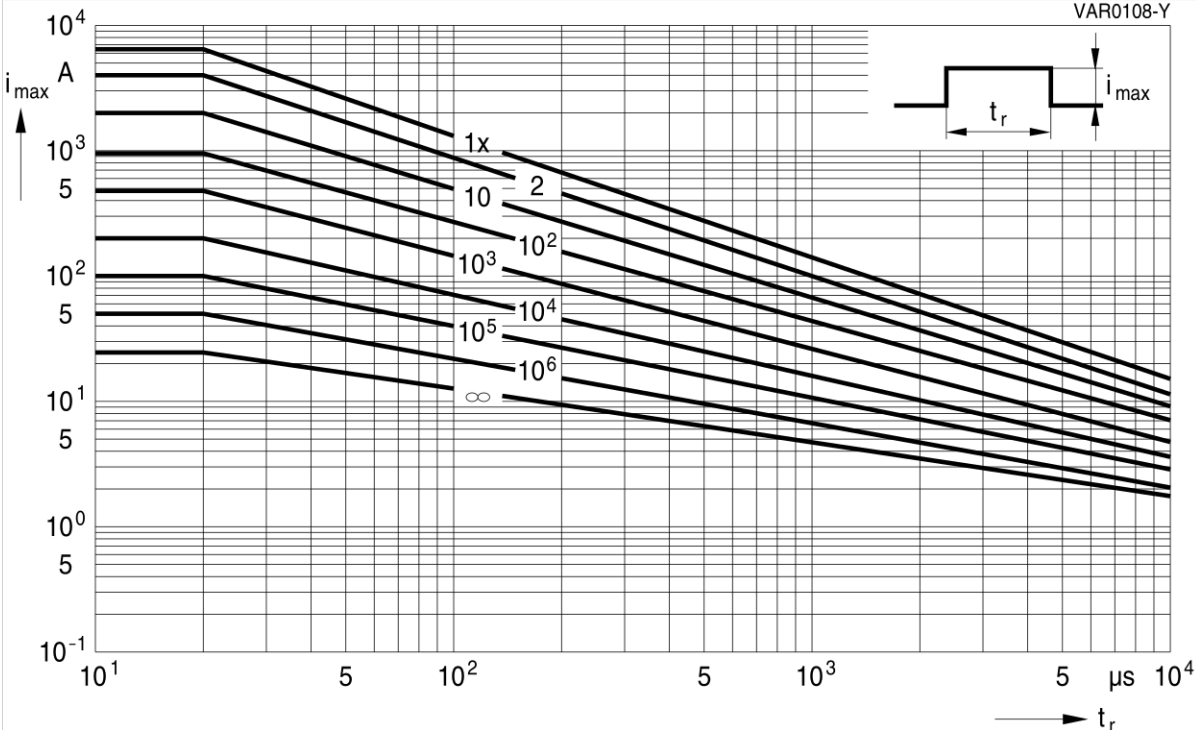
SIOV-S20K510 ... K1000
