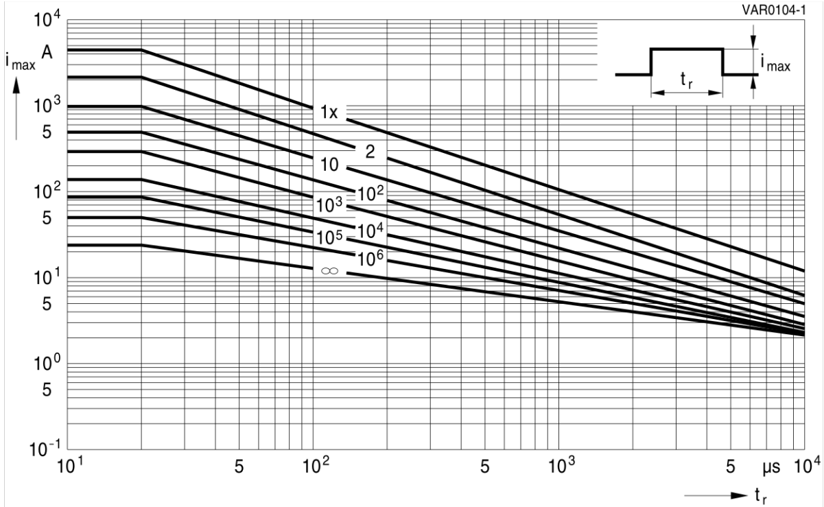
SIOV-S14K50 ... K320
