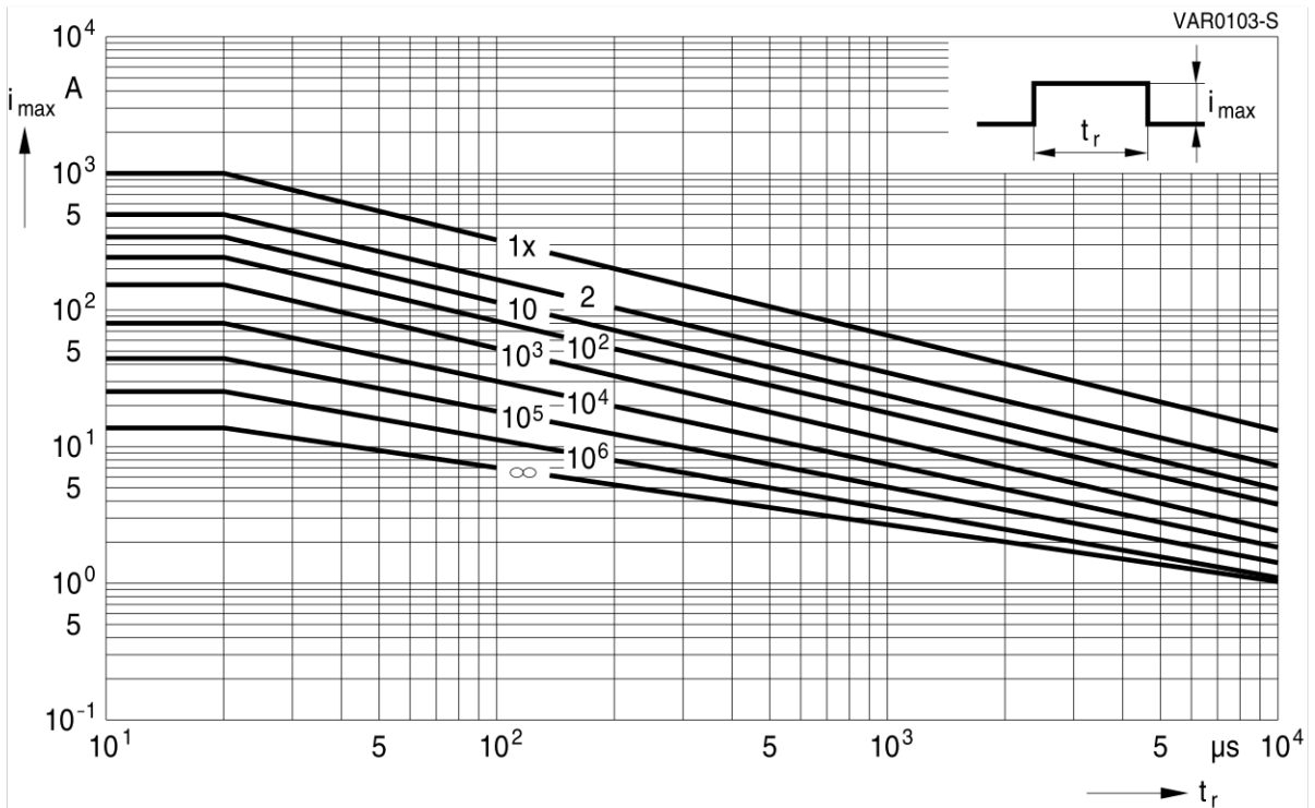
SIOV-S14K11 ... K40
