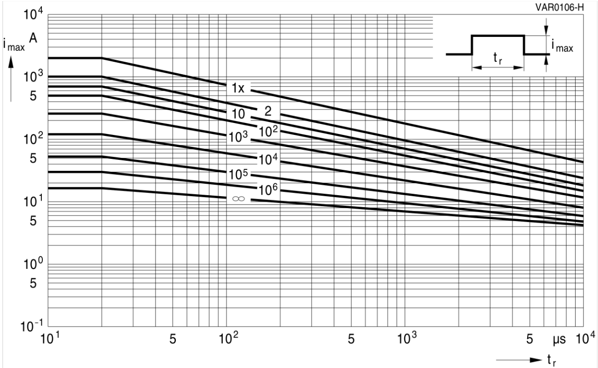
SIOV-S20K11 ... K40
