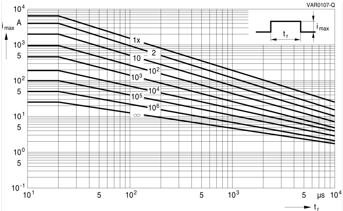
SIOV-S20K50 ... K115
