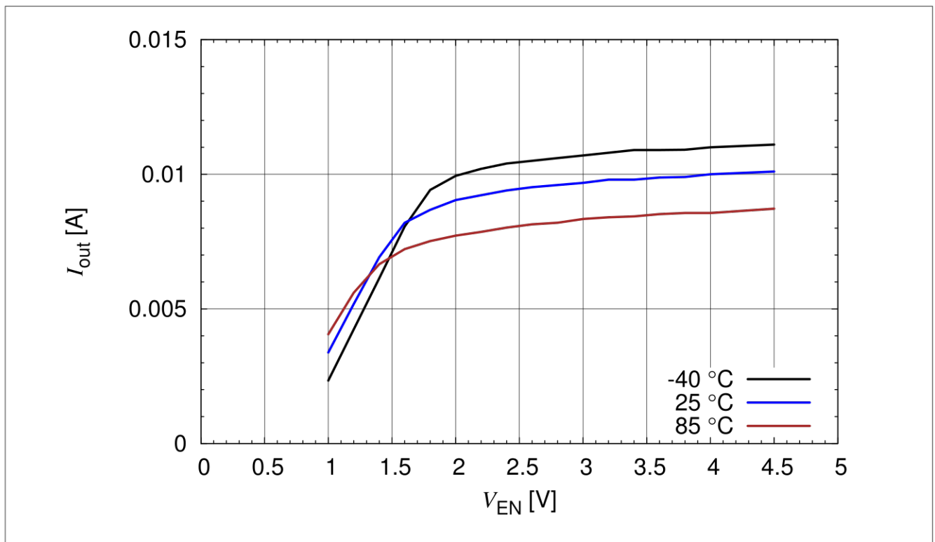
Figure 3-19 BCR 421U: Output Current versus V_{EN} I_{out} = f(V_{EN}) , V_{out} = 2 V, R_{ext} = \text{open} , T_A = \text{Parameter}
