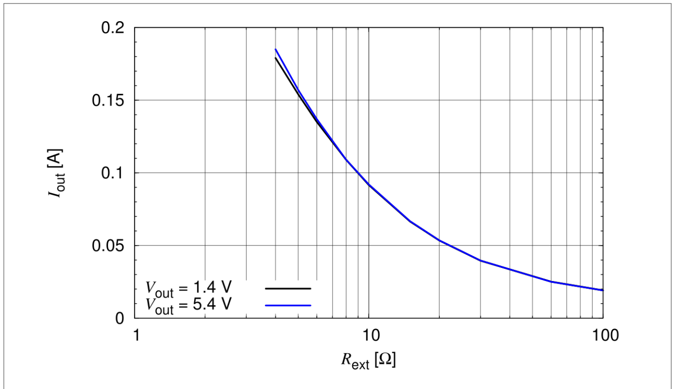
Figure 3-15 BCR 421U: Output Current versus R_{ext} I_{out} = f(R_{ext}) , V_{EN} = 3.3 \text{ V} , V_{out} = \text{Parameter}
