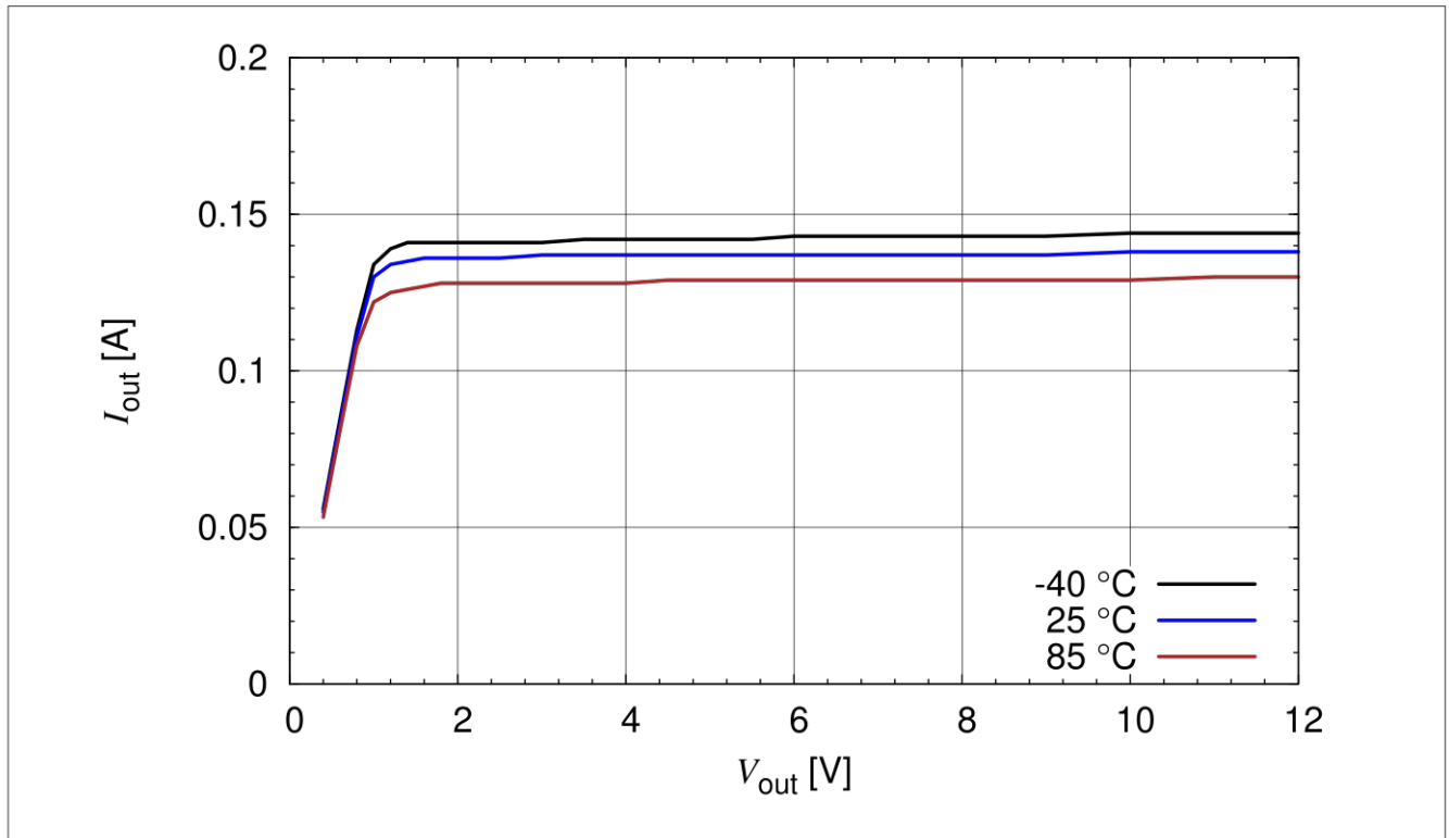
Figure 3-18 BCR 421U: Output Current versus V_{out} I_{out} = f(V_{out}) , V_{EN} = 3.3 V, R_{ext} = 6 \Omega , T_A = \text{Parameter}
