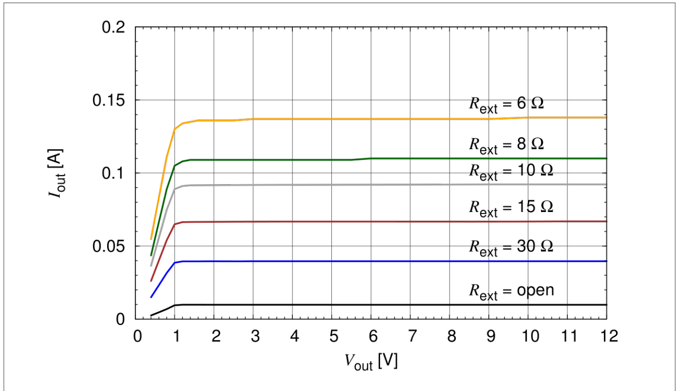
Figure 3-14 BCR 421U: Output Current versus V_{out} I_{out} = f(V_{out}) , V_{EN} = 3.3 \text{ V} , R_{ext} = \text{Parameter}
