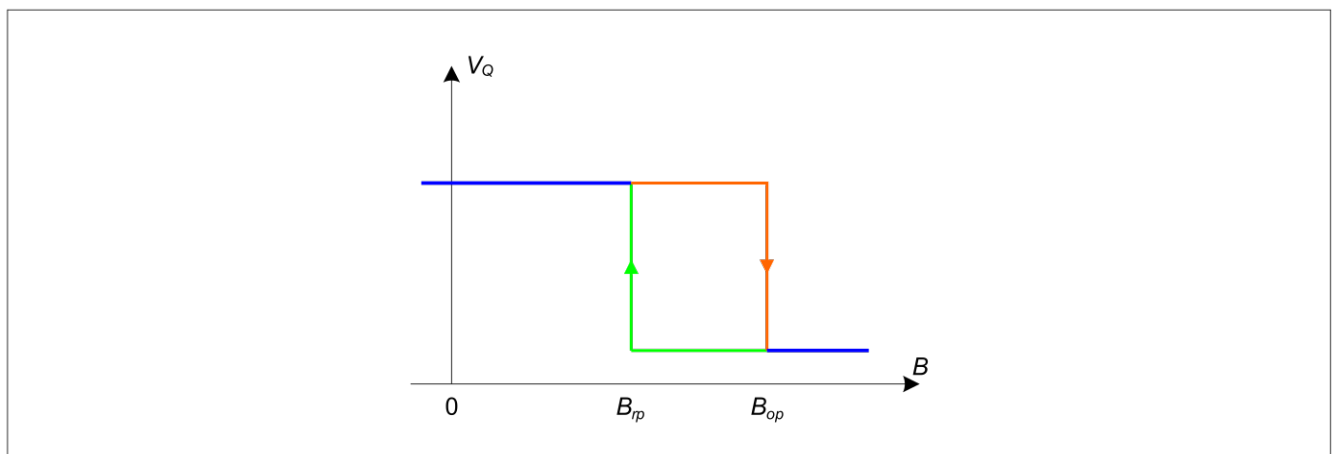
Figure 4 Output Signal
