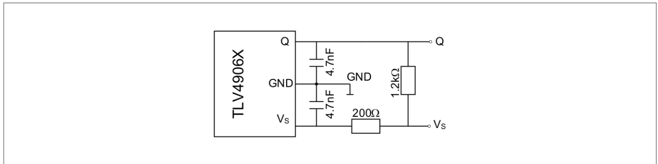
Figure 5 Application circuit
