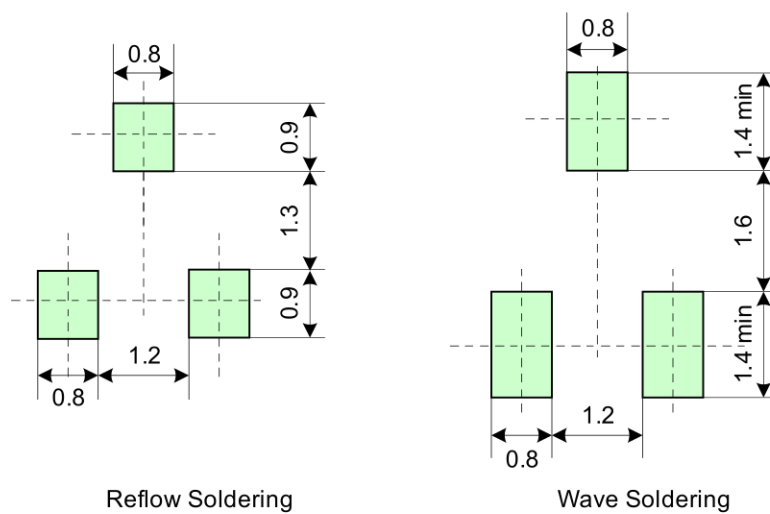
Figure 9 Footprint PG-SC59-3-5 (SOT23 compatible)
