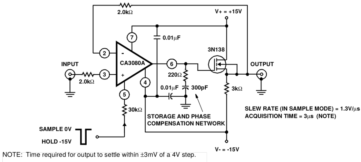
FIGURE 4. SCHEMATIC DIAGRAM OF THE CA3080A IN A SAMPLE-HOLD CONFIGURATION
