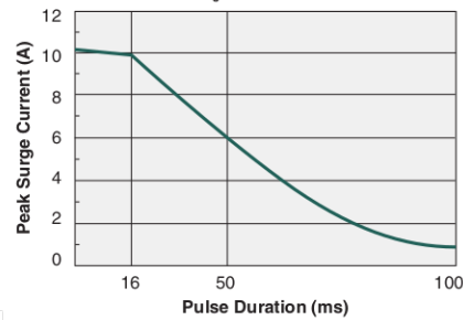
Maximum Surge Current (non-repetitive) (T J =50°C max)
