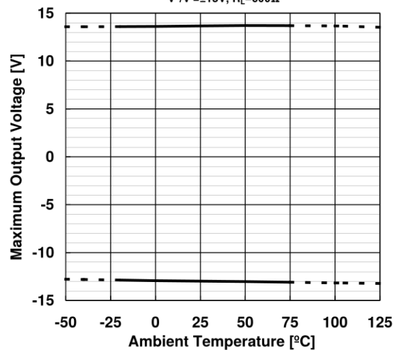
Maximum Output Voltage vs. Temperature V^+/V^-=\pm 15\text{V} , R_L=600\Omega
