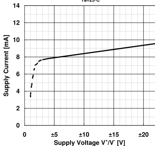
Supply Current vs. Supply Voltage T_a=25^\circ\text{C}
