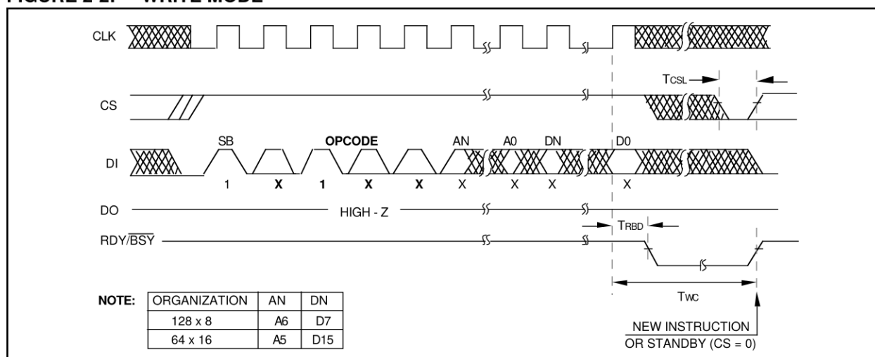
FIGURE 2-2: WRITE MODE
