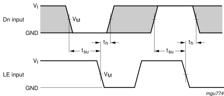
Measurement points are given in Table 8 . V OL and V OH are typical output voltage levels that occur with the output load. The shaded areas indicate when the input is permitted to change for predictable output performance.
