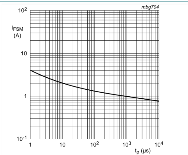
Fig. 3. Non-repetitive peak forward current as a function of pulse duration; typical values
