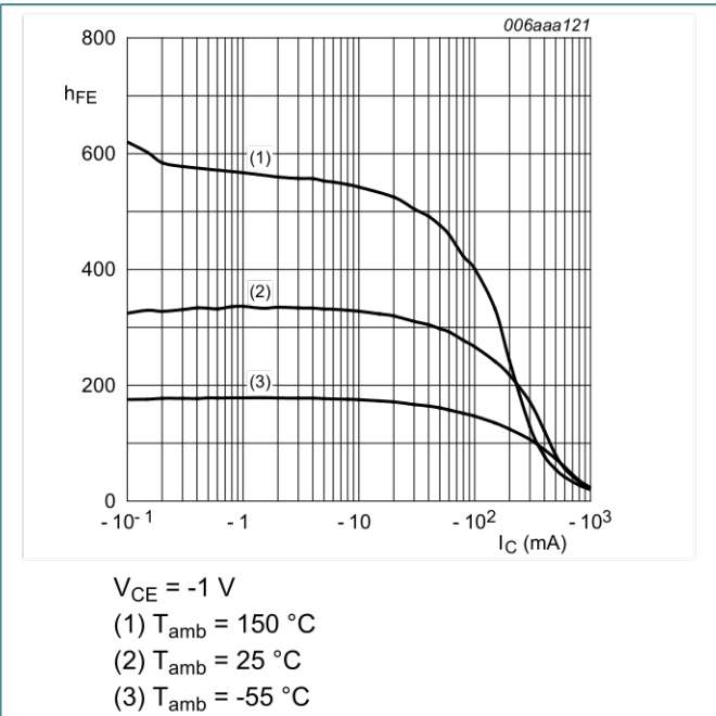
Fig. 12. BC807-40: DC current gain as a function of collector current; typical values
