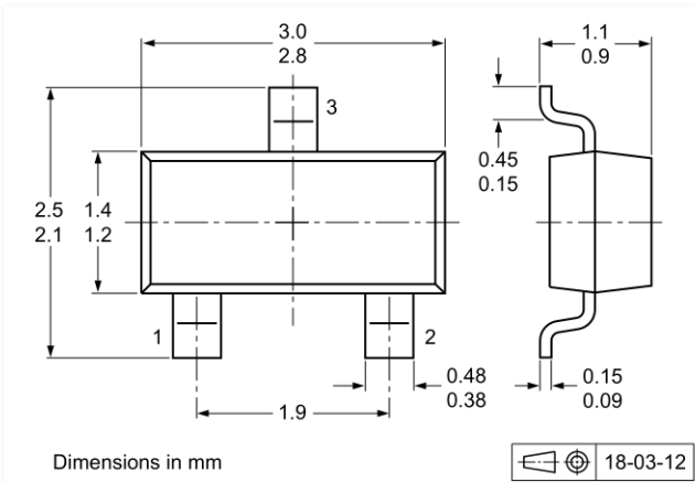
Fig. 16. Package outline SOT23 (TO-236AB)
