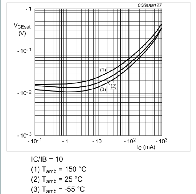
Fig. 14. BC807-40: Collector-emitter saturation voltage as a function of collector current; typical values
