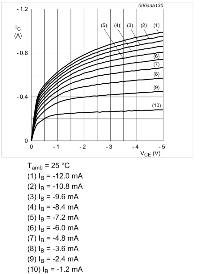
Fig. 15. BC807-40: Collector current as a function of collector-emitter voltage; typical values
