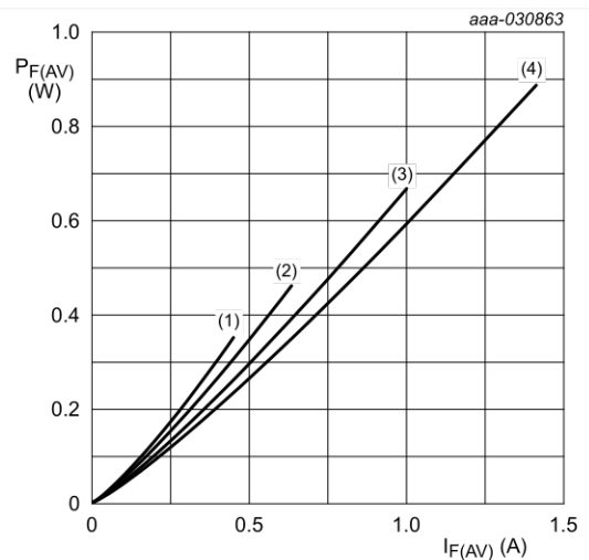
T_j = 175\text{ °C} (1) \delta = 0.1 (2) \delta = 0.2 (3) \delta = 0.5 (4) \delta = 1 ; DC
