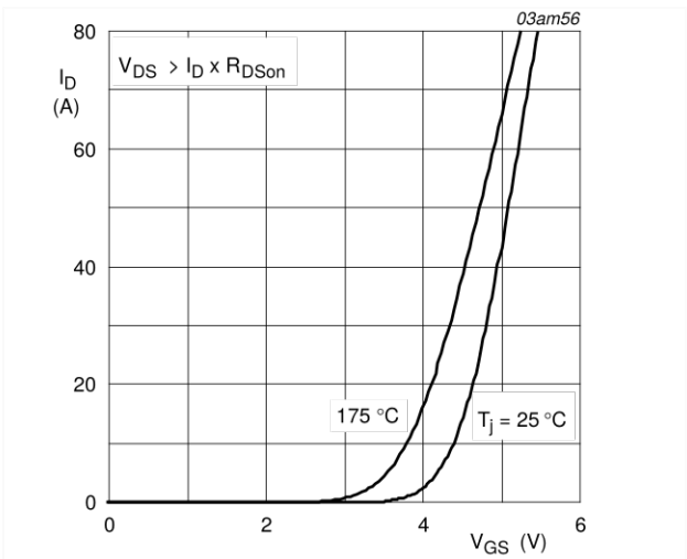
Fig 6. Transfer characteristics: drain current as a function of gate-source voltage; typical values
