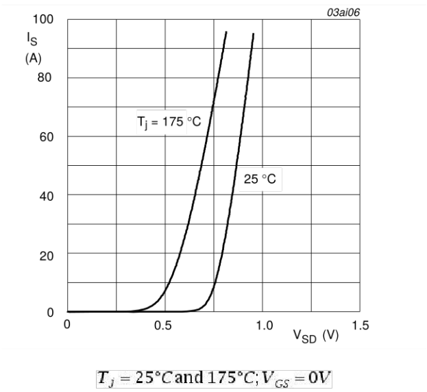
Fig 13. Source current as a function of source-drain voltage; typical values
