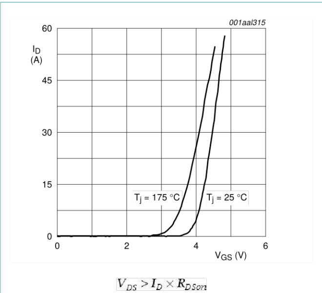
Fig 5. Transfer Characteristic: drain current as a function of gate-source voltage; typical values
