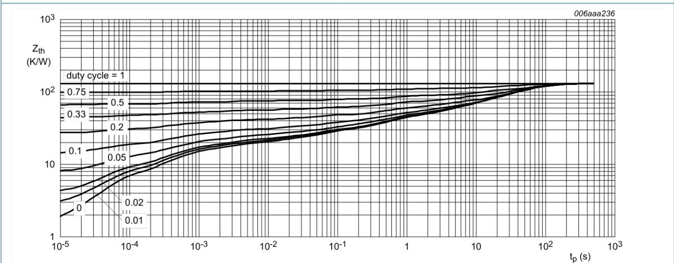
Fig. 2. Transient thermal impedance as a function of pulse time; typical values
