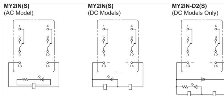
Terminal Arrangement/Internal Connections (Bottom View)
