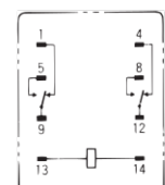
Terminal Arrangement/Internal Connections (Bottom View) Standard Models
