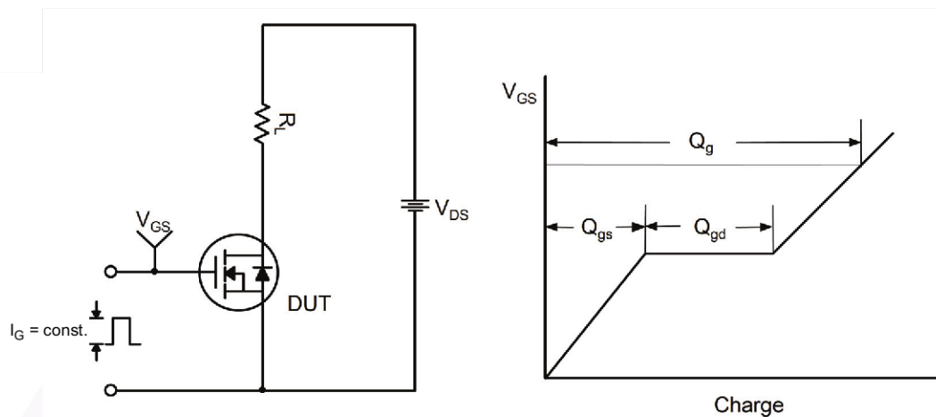
Figure 11. Gate Charge Test Circuit & Waveform
