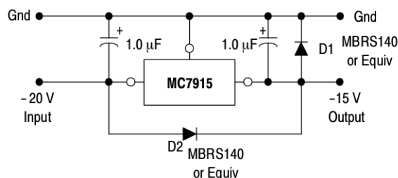
Figure 11. Protection Diodes
