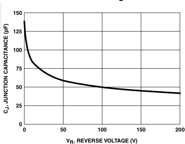
Figure 7. Junction Capacitance vs Reverse Voltage
