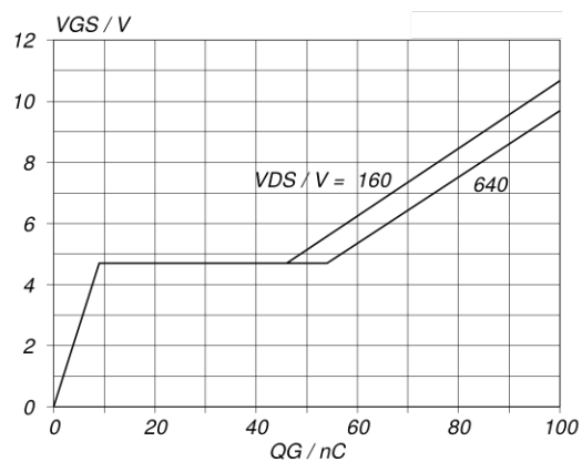
Fig.13. Typical turn-on gate-charge characteristics. V_{GS} = f(Q_G) ; conditions: I_D = 7.6 A; parameter V_{DS}
