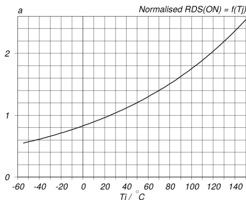
Fig. 9. Normalised drain-source on-state resistance. a = R_{DS(ON)}/R_{DS(ON)25 \text{ }^\circ\text{C}} = f(T_j) ; I_D = 4 \text{ A} ; V_{GS} = 10 \text{ V}
