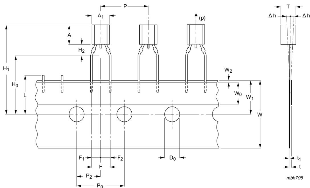
Fig 5. Configuration of bandolier: spread leads
