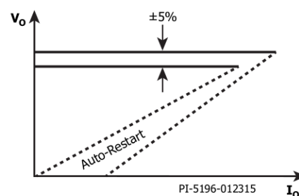
(b) Output Characteristic Envelope
