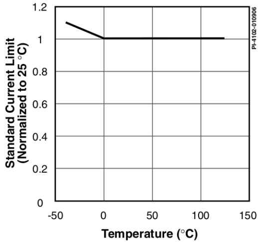
Figure 20. Standard Current Limit vs. Temperature.
