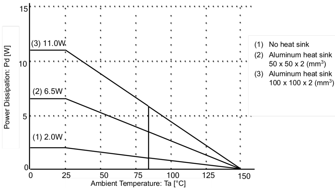
Figure 17. Power Dissipation
