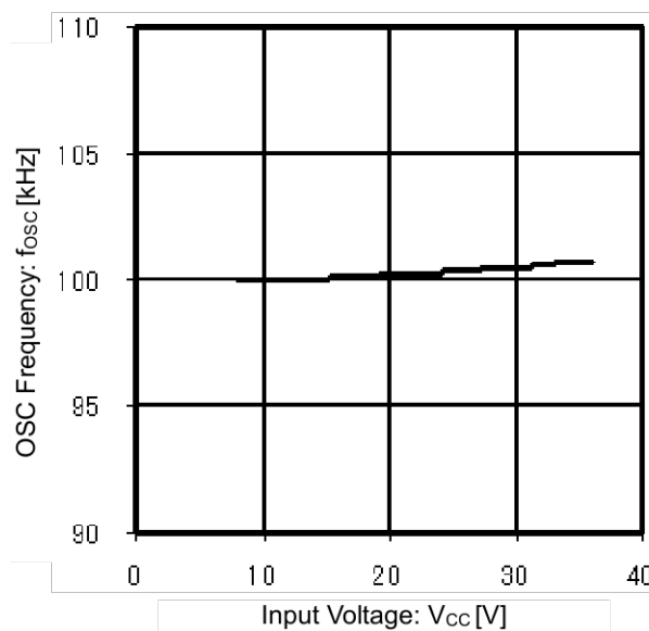
Figure 10. OSC Frequency vs Input Voltage
