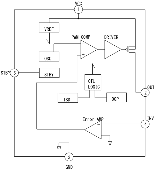
Figure 2. Block Diagram
