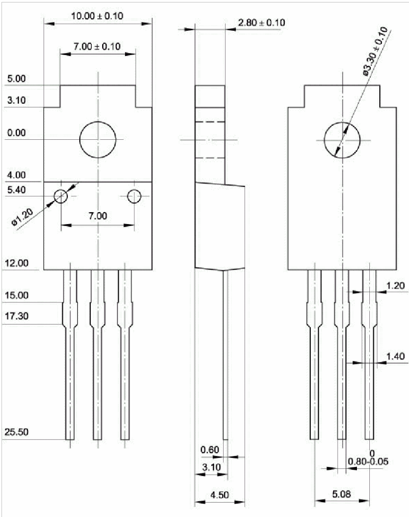
Fig.2 Outline dimensions (unindicated tolerance:±0.15 mm)
