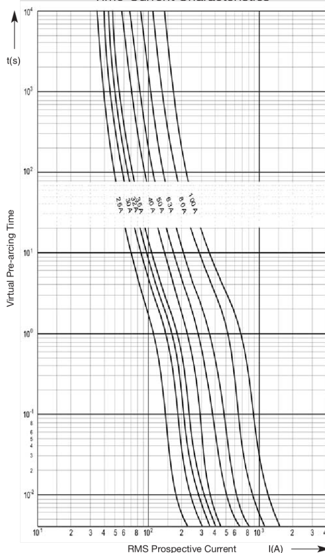
Time-Current Characteristics
