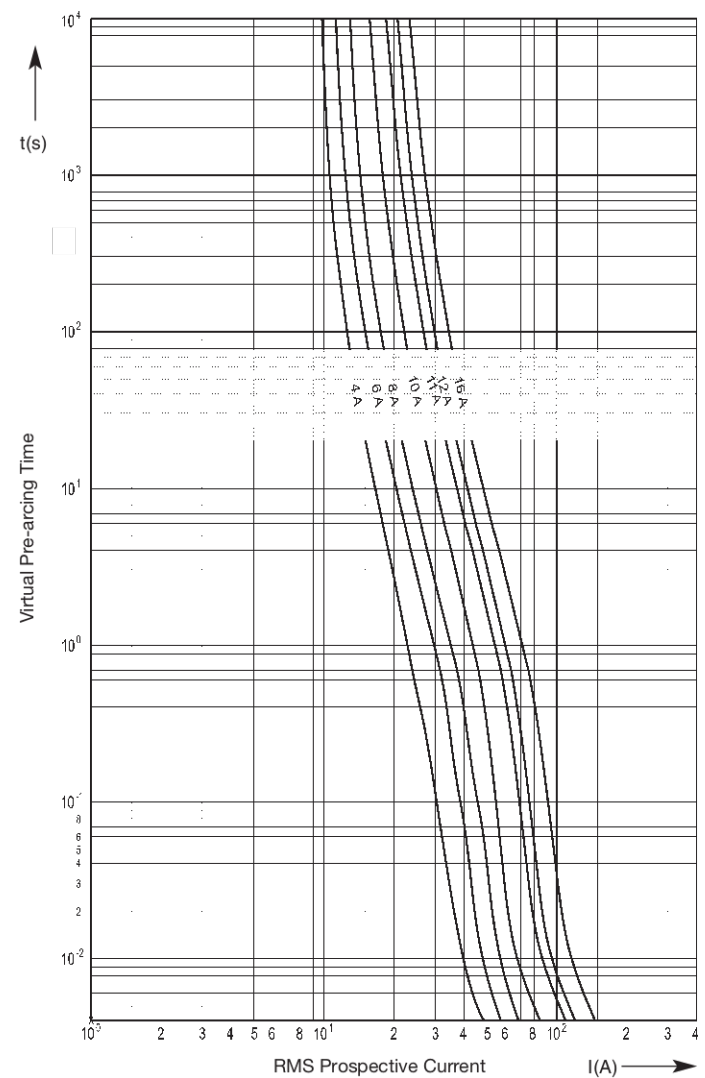
Time-Current Characteristics
