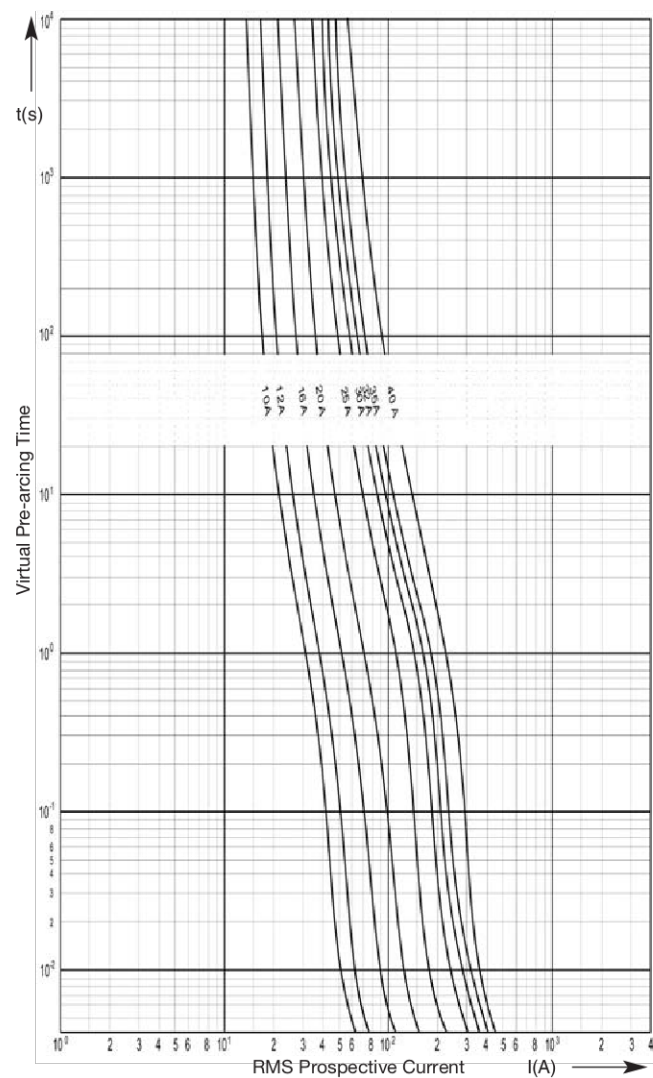
Time-Current Characteristics
