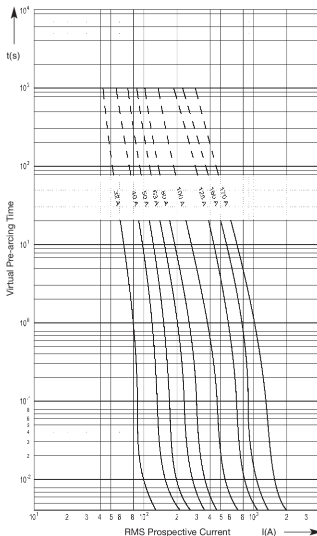
Time-Current Characteristics
