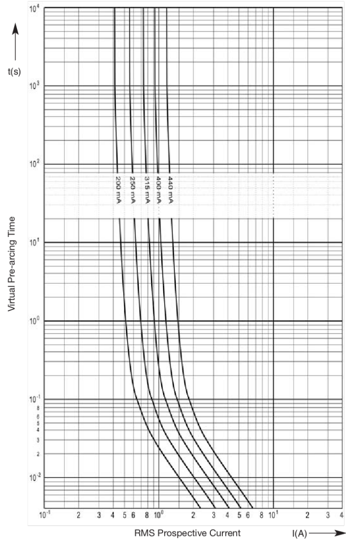
Time-Current Characteristics
