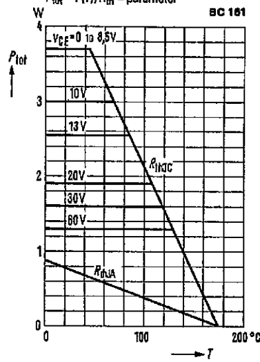
Total power dissipation versus temperature P_{tot} = f(T); R_{th} = \text{parameter}
