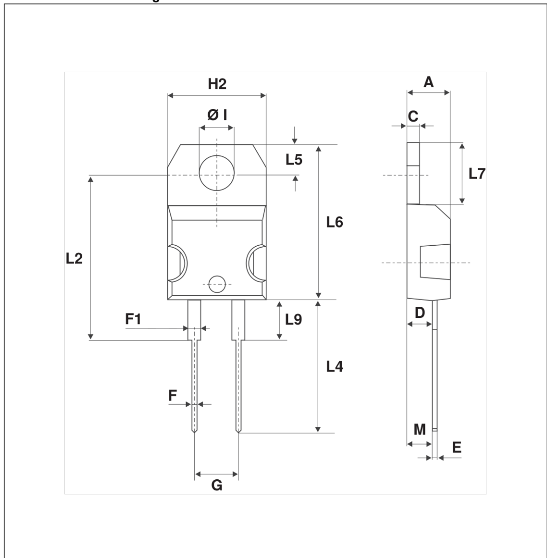
Figure 11. T0-220AC dimension definitions
