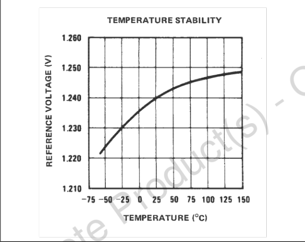
Figure 9. Temperature stability
