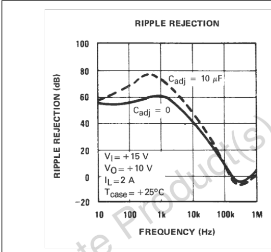
Figure 13. Ripple rejection
