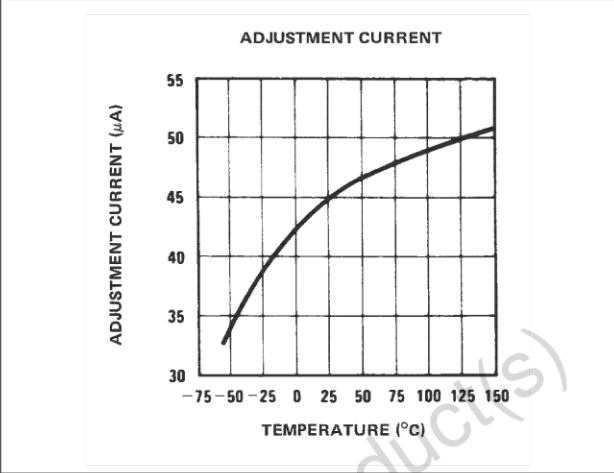
Figure 8. Adjustment current
