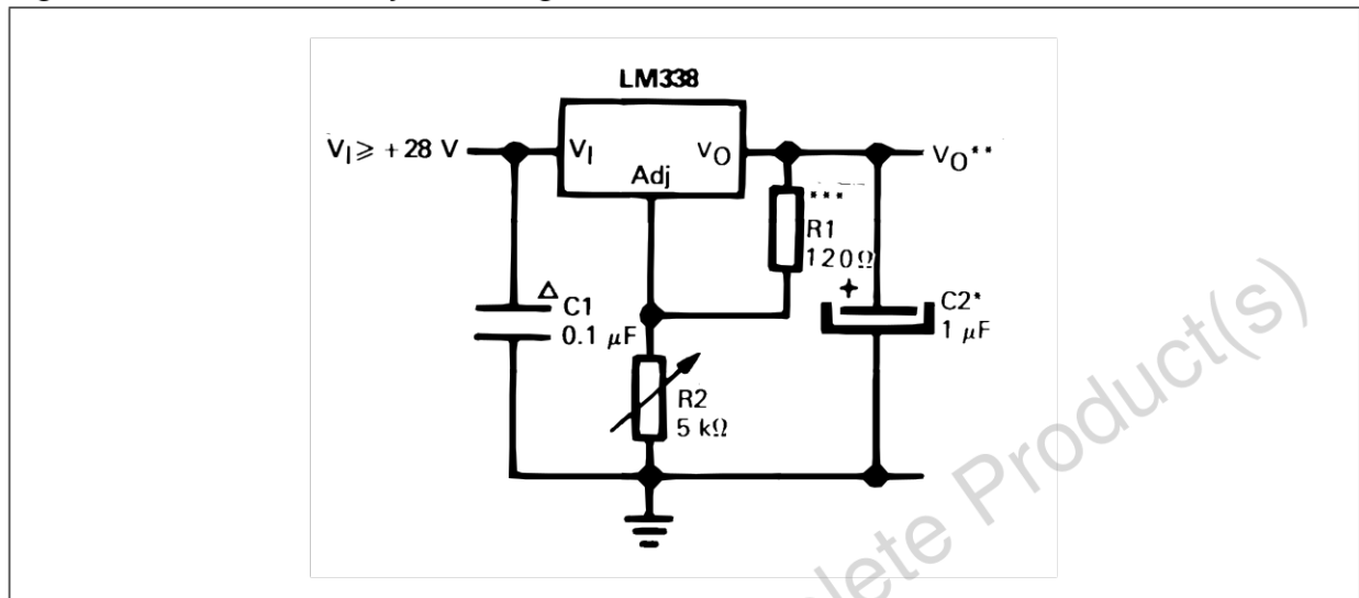
Figure 17. 1.2 V to 25 V adjustable regulator
