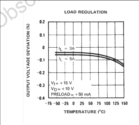
Figure 6. Load regulation
