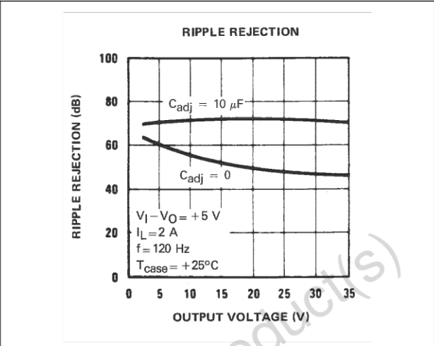
Figure 14. Ripple rejection
