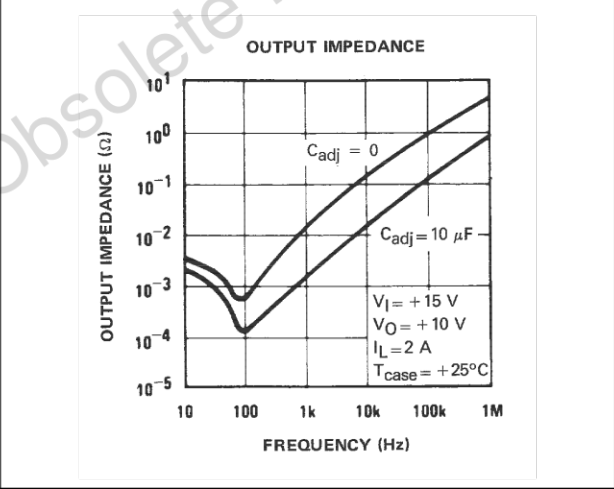
Figure 10. Output impedance
