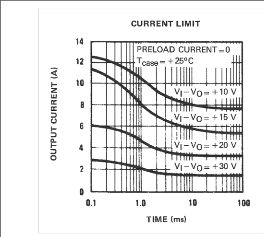
Figure 5. Current limit
