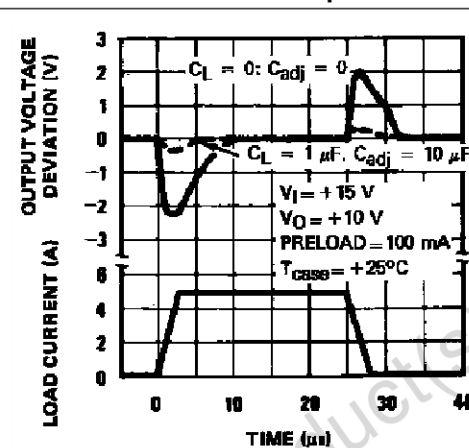
Figure 16. Load transient response
