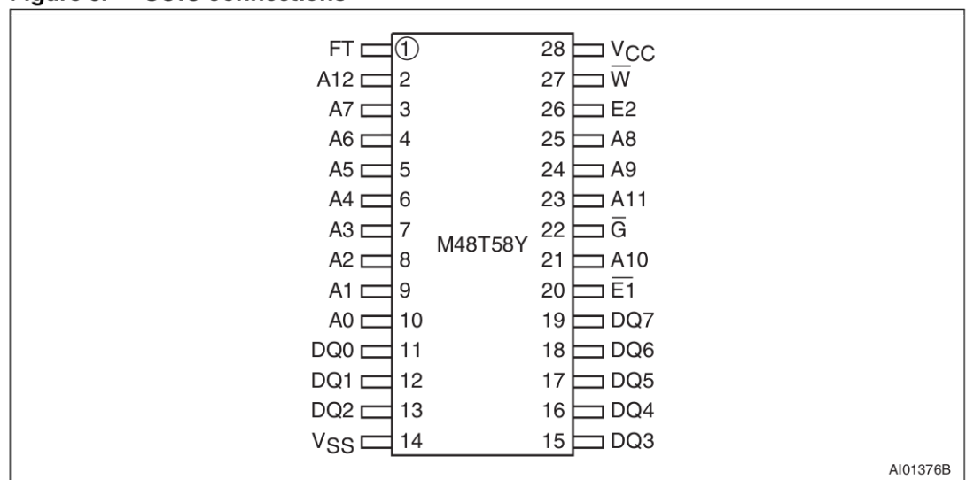
Figure 3. SOIC connections
