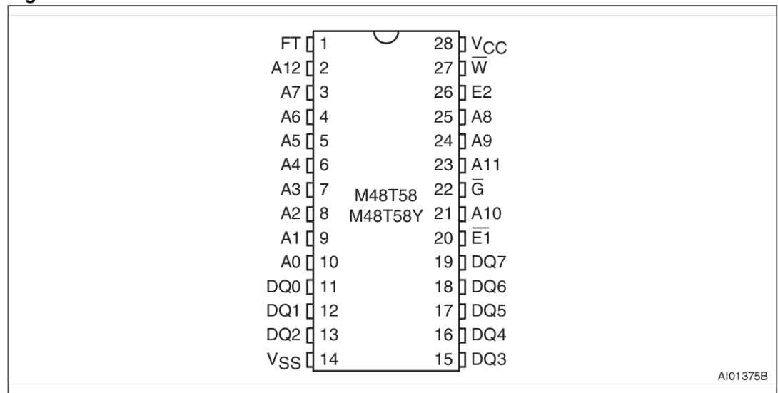
Figure 3. SOIC connections
