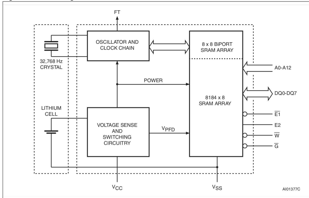
Figure 4. Block diagram
