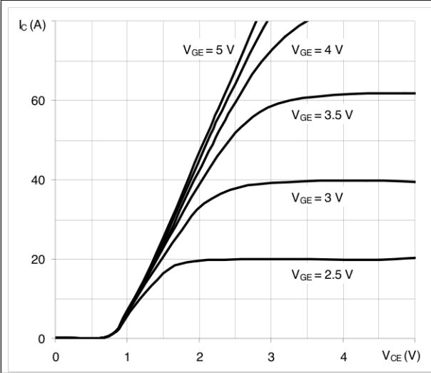
Figure 4. Output characteristics ( T_J = 25 °C)
