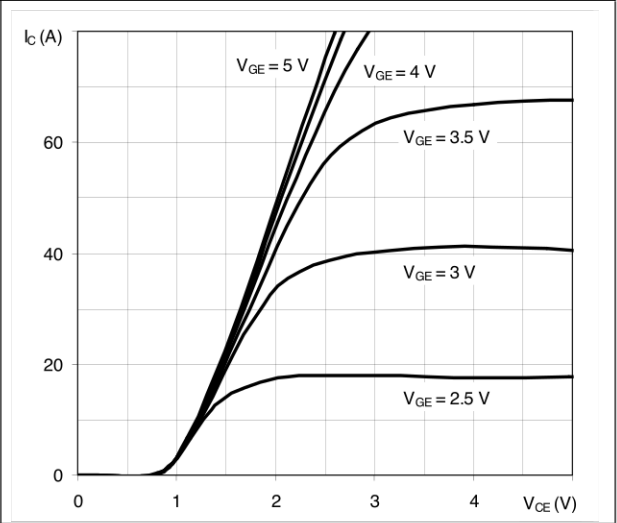
Figure 5. Output characteristics ( T_J = -40 °C)
