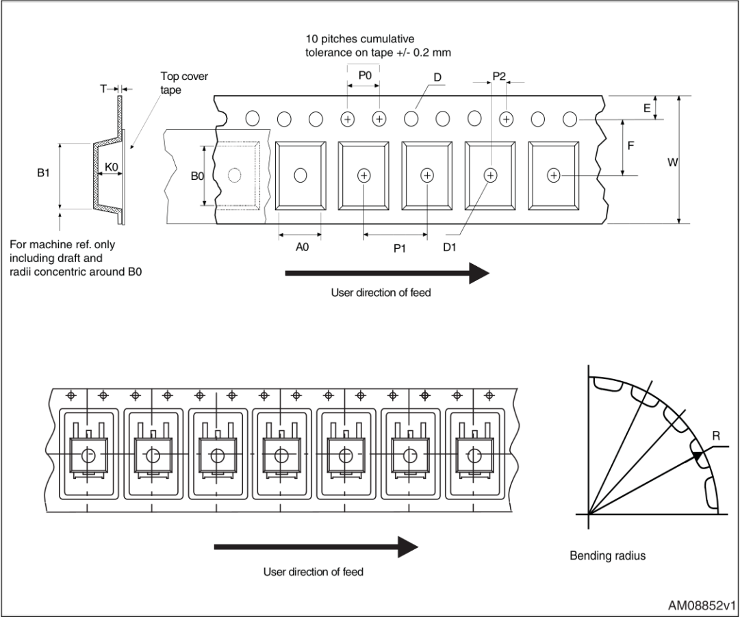
Figure 20. Tape for D 2 PAK (TO-263)
