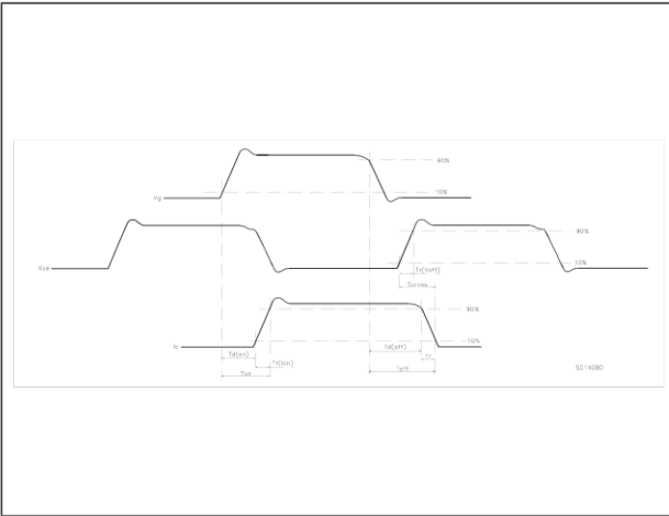
Figure 20. Switching waveforms
