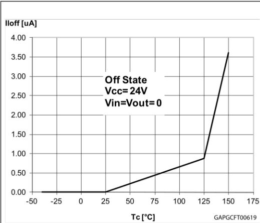
Figure 13. Off-state output current
