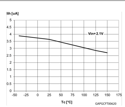
Figure 14. High level input current
