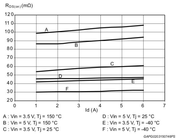
Figure 21. Static drain source on-resistance vs drain current
