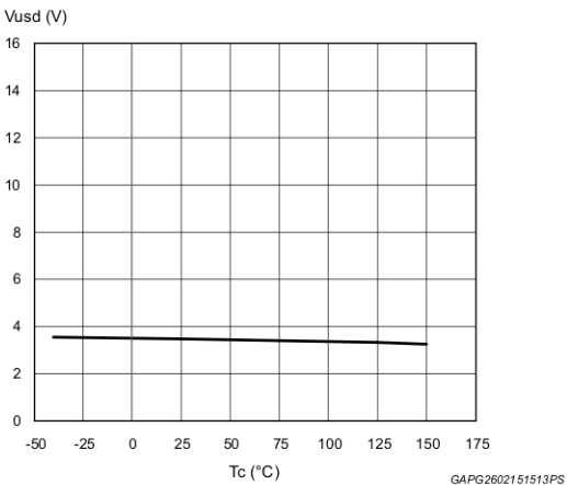
Figure 14. Undervoltage shutdown
