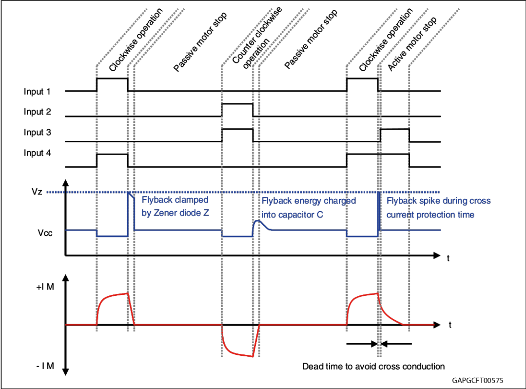
Figure 27. Recommended motor operation
