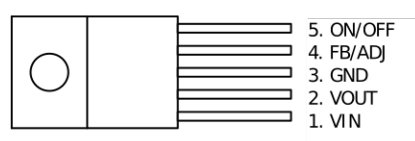
TO-220
