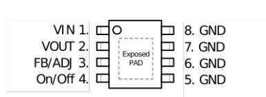
SOP-8PP
