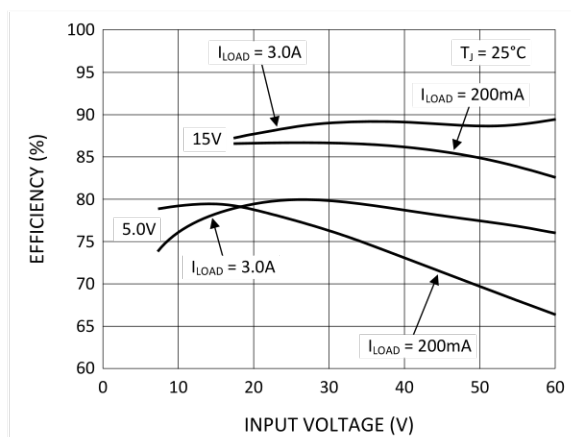
Figure 9. Efficiency
