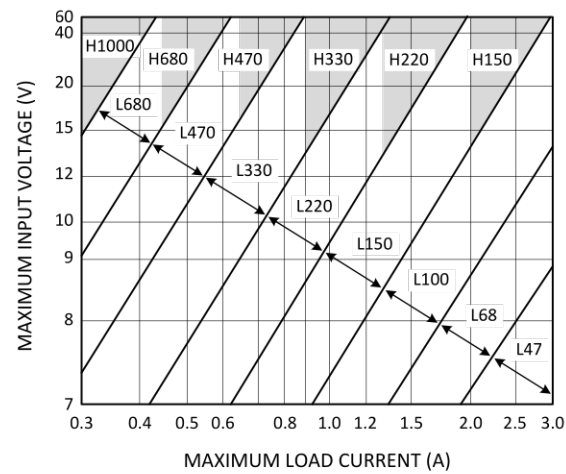
Figure 22. LM2576HV-5.0
