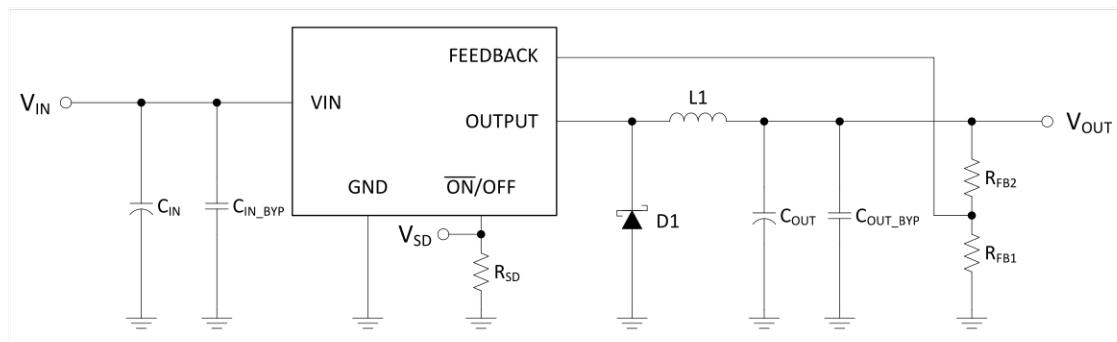
Figure 27. Schematic for PCB Layout Example
