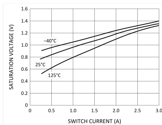
Figure 8. Switch Saturation Voltage
