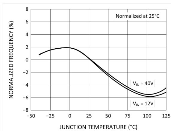
Figure 7. Oscillator Frequency
