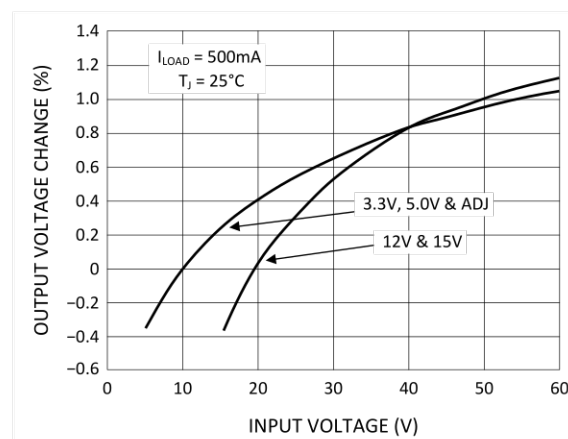
Figure 2. Line Regulation
