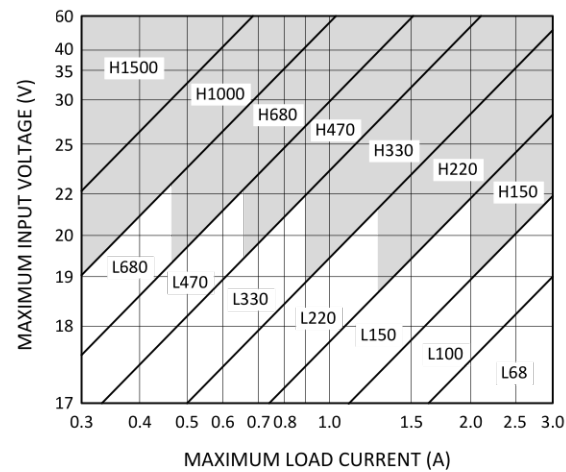
Figure 24. LM2576HV-15
