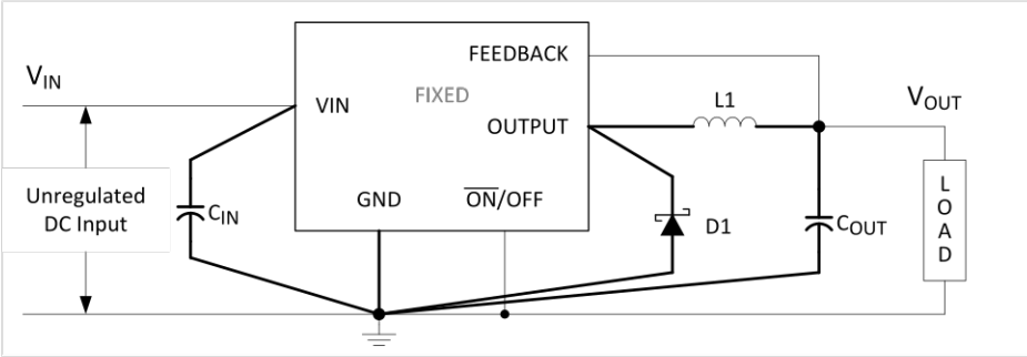
Figure 19. Fixed Output Voltage Version
