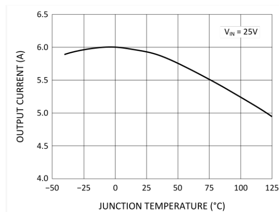
Figure 4. Current Limit
