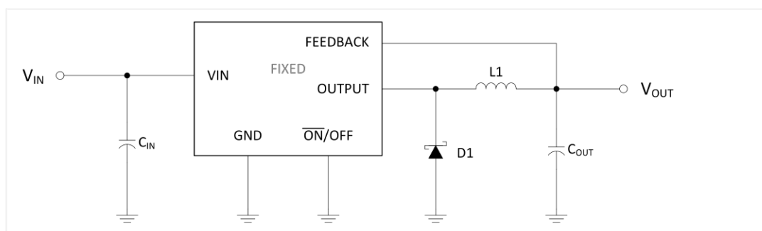
&lt; Fixed Output Voltage Version &gt;
