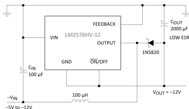
Figure 14. Negative Boost
