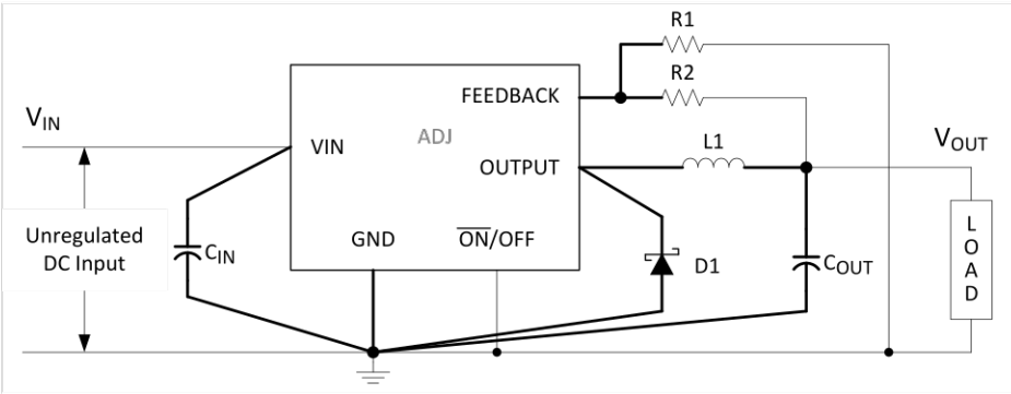
Figure 20. Adjustable Output Voltage Version
