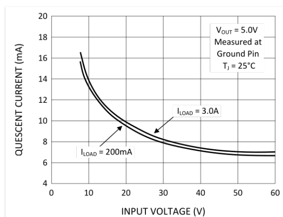
Figure 5. Quiescent Current
