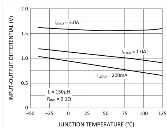
Figure 3. Dropout Voltage
