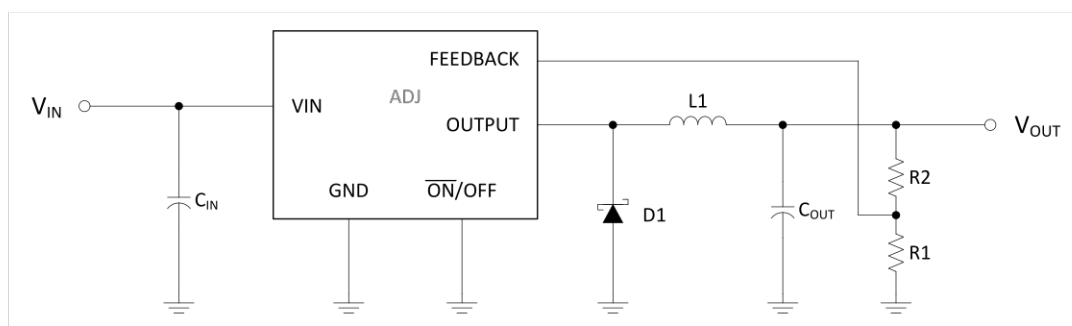
&lt; Adjustable Output Voltage Version &gt;
