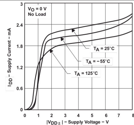
Figure 36. TLC2272 Supply Current vs Supply Voltage
