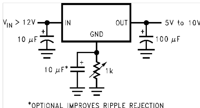
Figure 19. Adjustable Fixed Regulator
