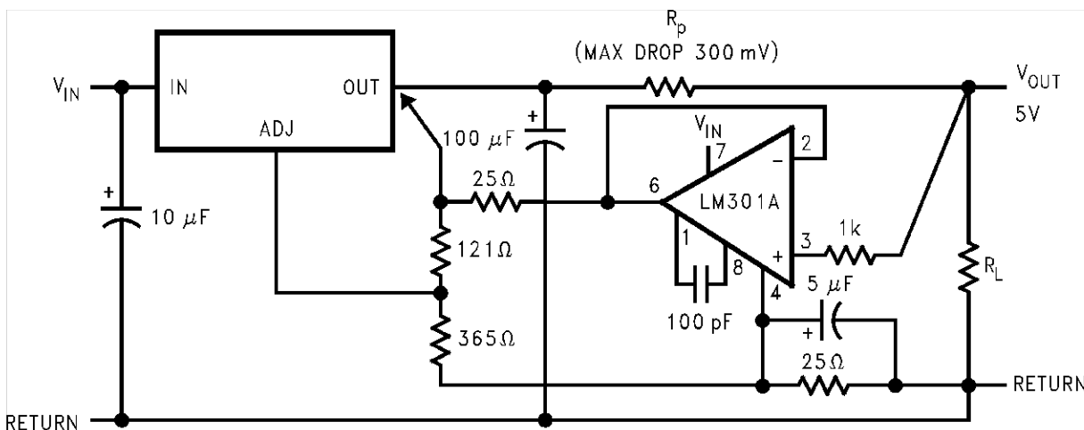
Figure 26. Remote Sensing
