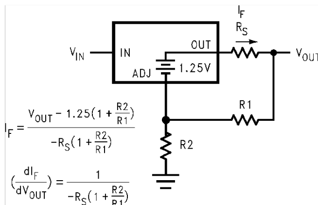
Figure 18. Battery Charger
