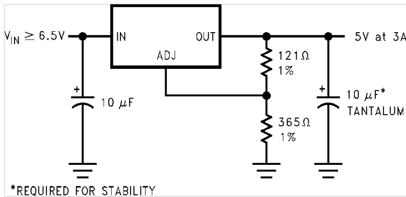
Figure 16. Adjustable @ 5V
