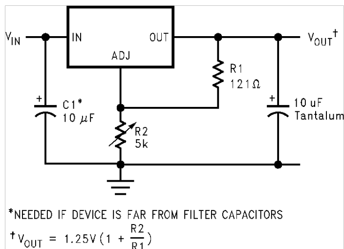
Figure 15. 1.2-V to 15-V Adjustable Regulator
