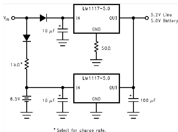
Figure 9-7. Battery Backed-Up Regulated Supply
