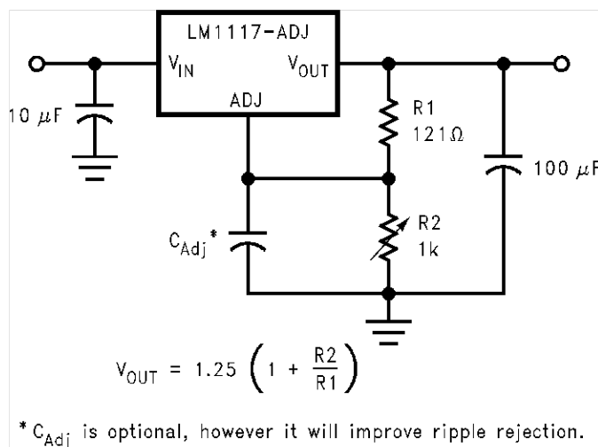
Figure 9-1. 1.25-V to 10-V Adjustable Regulator With Improved Ripple Rejection
