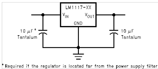
Figure 9-3. Fixed Output Regulator
