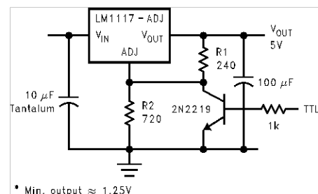
Figure 9-6. 5-V Logic Regulator With Electronic Shutdown*
