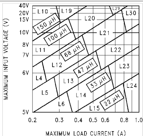
Figure 27. LM2595 3.3-V
