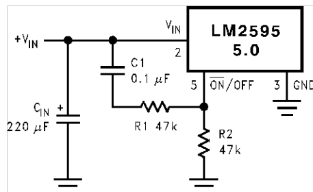
Figure 14. Delayed Start-Up
