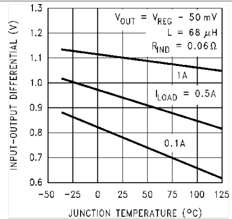
Figure 6. Dropout Voltage
