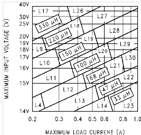
Figure 29. LM2595 12-V
