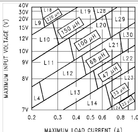
Figure 28. LM2595 5-V
