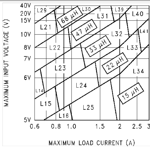
Figure 27. LM2596-3.3
