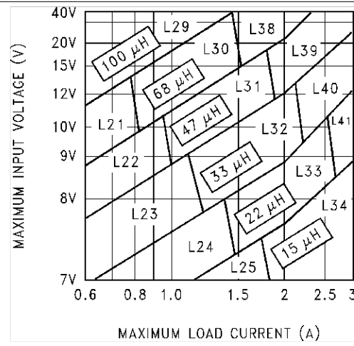
Figure 28. LM2596-5.0
