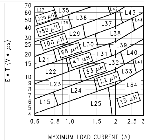
Figure 30. LM2596-ADJ
