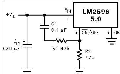
Figure 14. Delayed Start-Up
