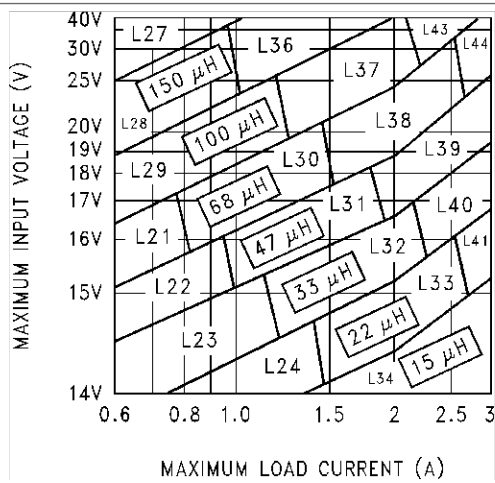
Figure 29. LM2596-12
