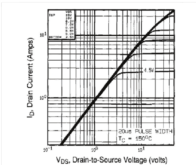
Fig. 2 - Typical Output Characteristics, T_C = 150^\circ\text{C}
