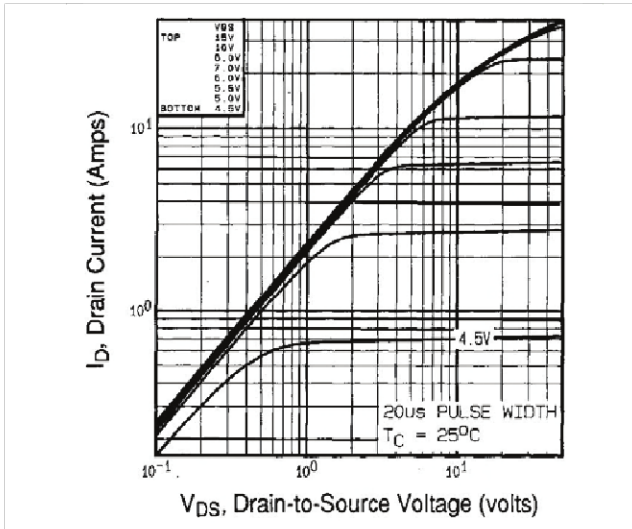
Fig. 1 - Typical Output Characteristics, T_C = 25^\circ\text{C}
